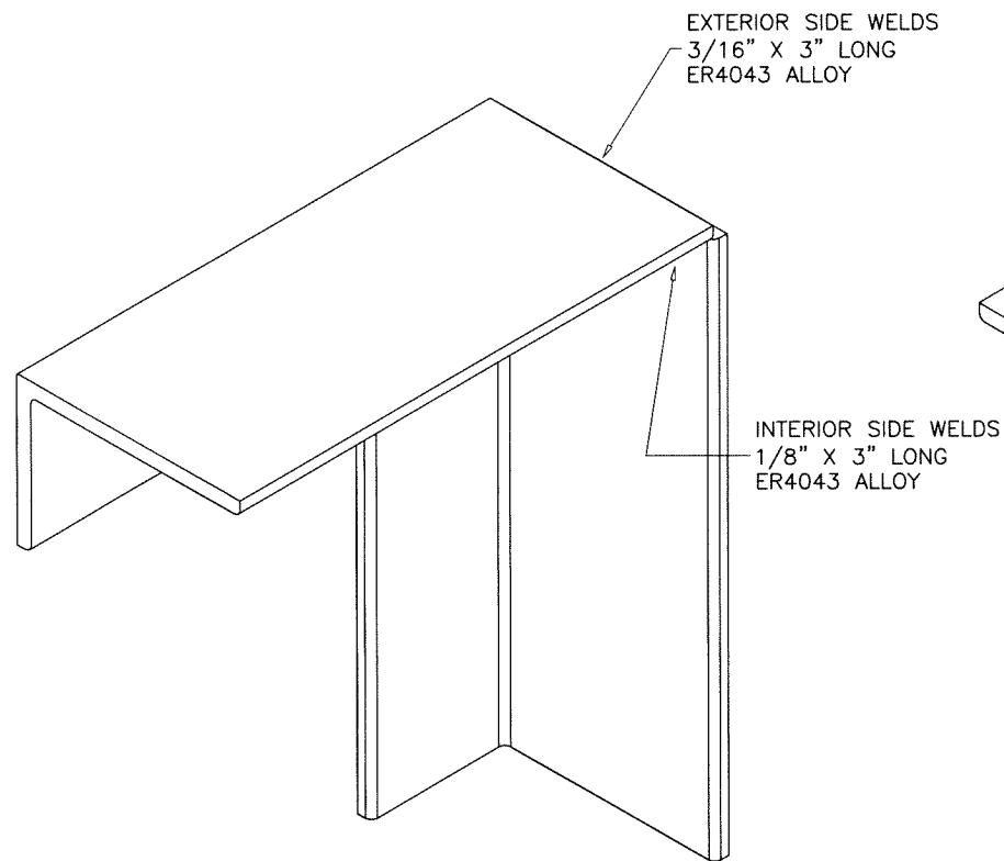
WINDOW CORNER
