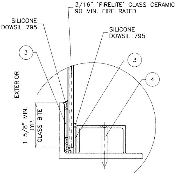
GLAZING DETAIL
